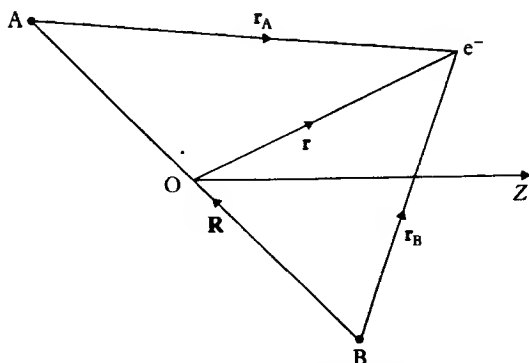
13.9 A coordinate system for the discussion of an H^+ + H collision. Note that the position vector r of the electron can be in any direction whereas the vector R lies in the plane of motion of A and B, which has been taken to be the XZ plane (see Fig. 13.8).
